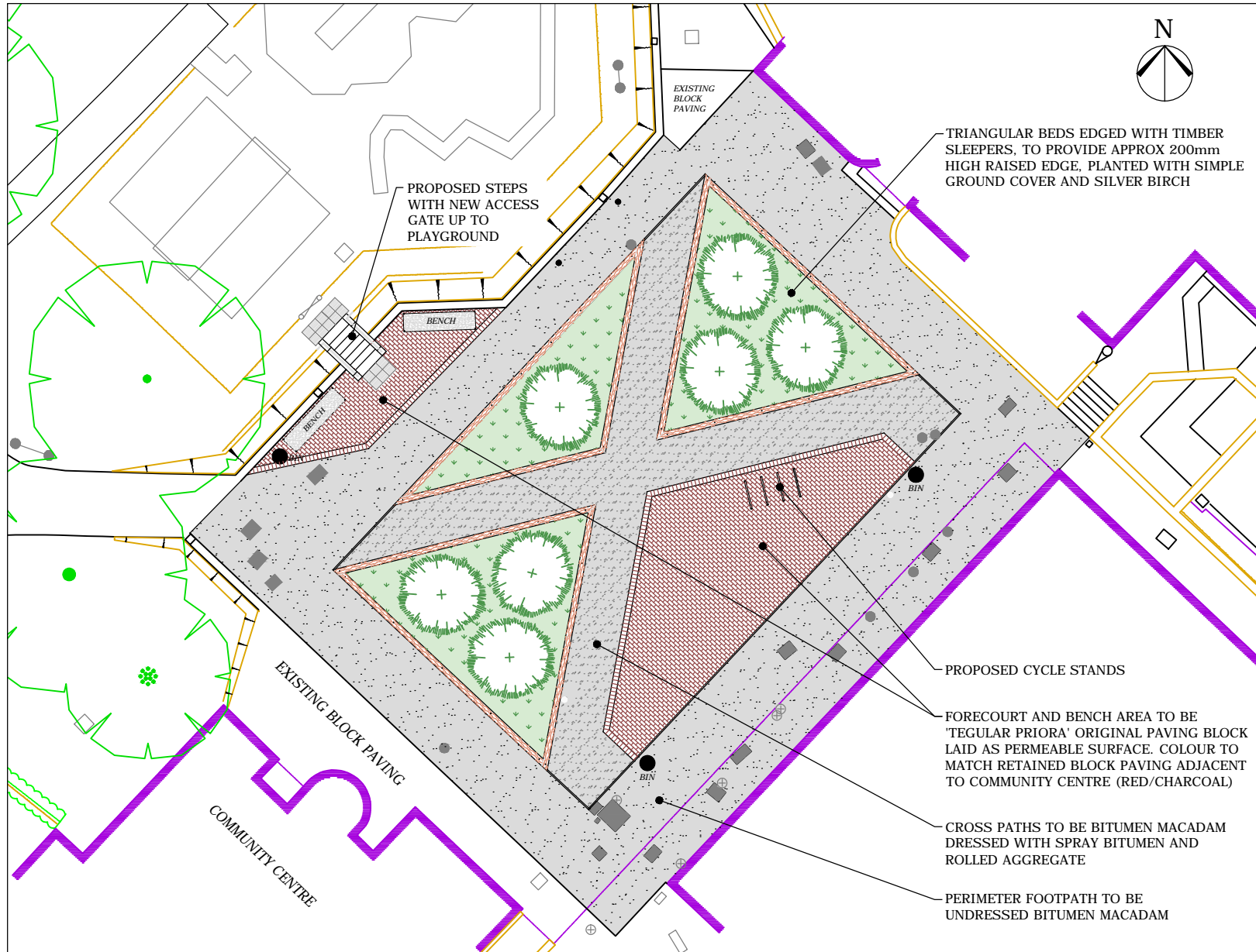
LANDSCAPE PROPOSAL SCALE 1:75
